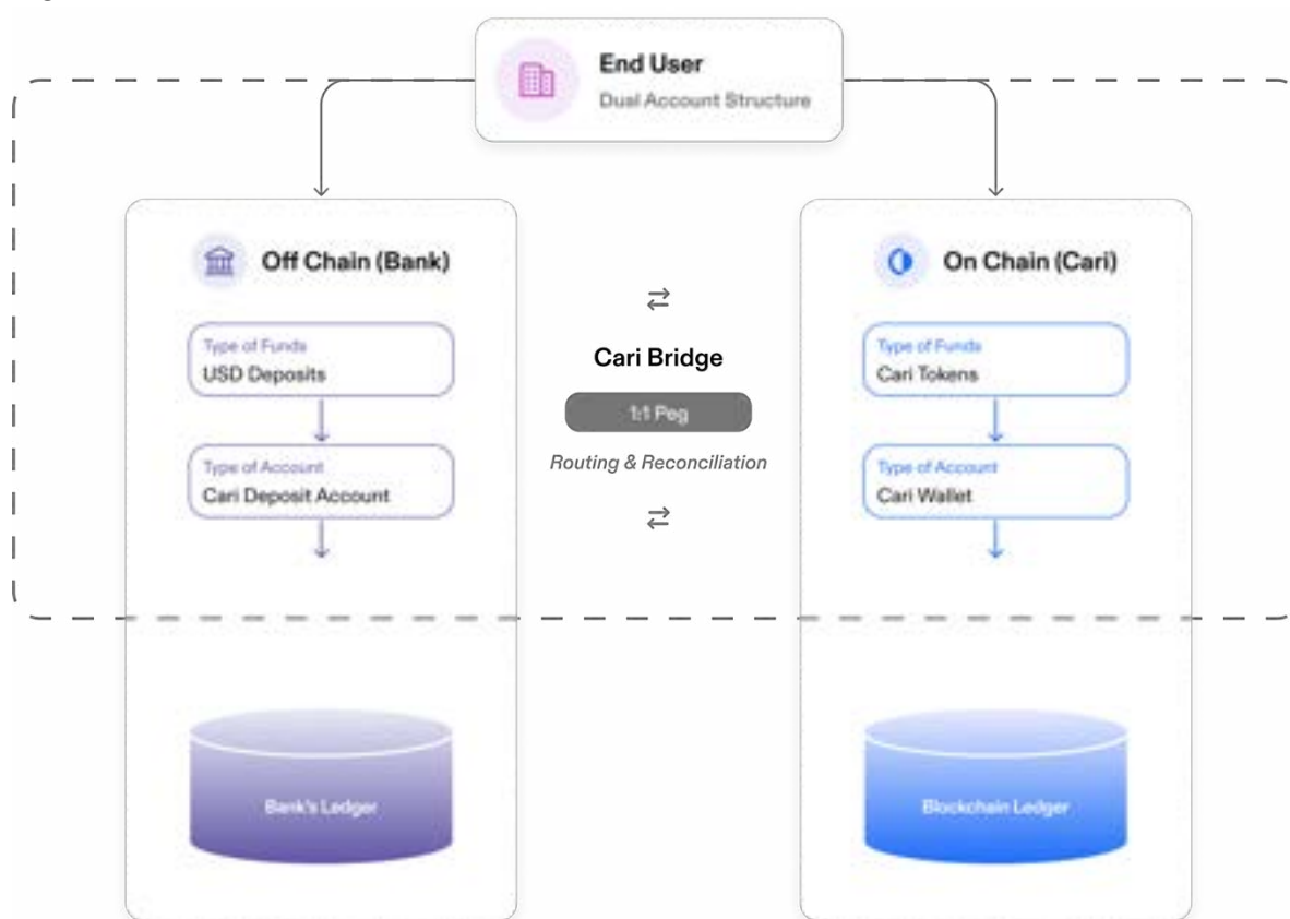
Figure 5: End User’s Dual Account Structure
