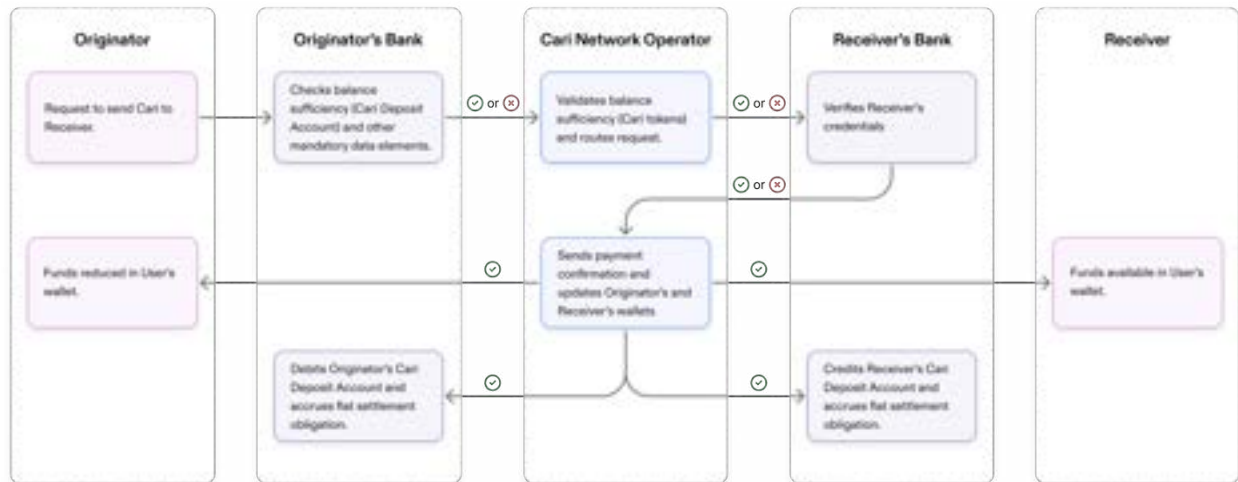
Figure 9: Basic Flow - Transferring Cari
